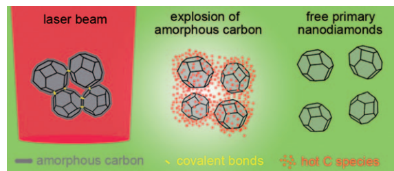
Scheme 1. Deaggregation of DNDs by laser irradiation in liquid.
